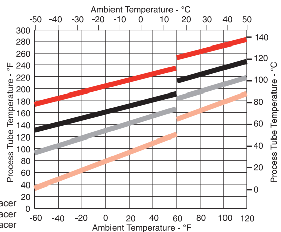
TPE2 - TWO 1/2" (12mm) PROCESS LINES WITH HIGH TEMPERATURE TRACER
