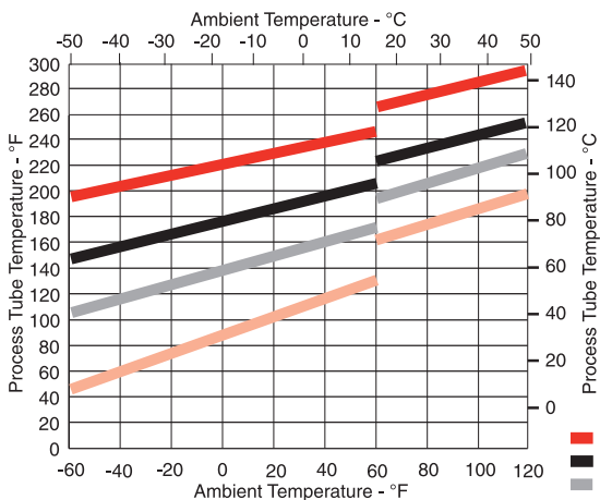
TPE1 - ONE 1/2" (12mm) PROCESS LINE WITH HIGH TEMPERATURE TRACER
