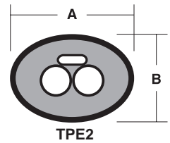
TPE2 - TWO 1/2" (12mm) PROCESS LINES WITH LOW TEMPERATURE TRACER
