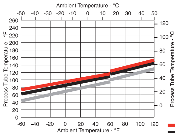
TPE1 - ONE 1/2" (12mm) PROCESS LINE WITH LOW TEMPERATURE TRACER
