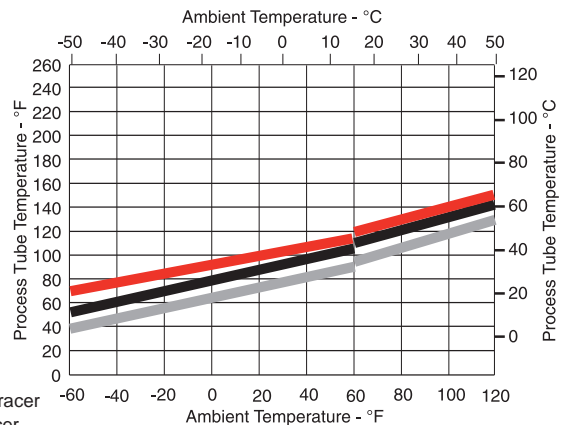
TPE2 - TWO 1/2" (12mm) PROCESS LINES WITH LOW TEMPERATURE TRACER
